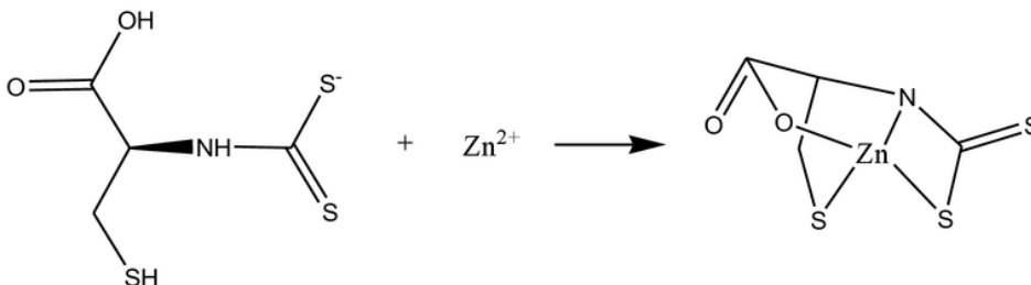
Figure 1. Synthesis reaction of Zn(II) cysteine dithiocarbamate
