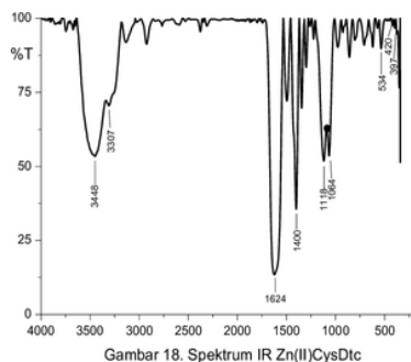
Figure 3. IR Spectrum of Zn(II) cysteine dithiocarbamate
