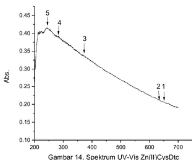
Figure 2. UV-Vis Spectrum of Zn(II) cysteine dithiocarbamate
